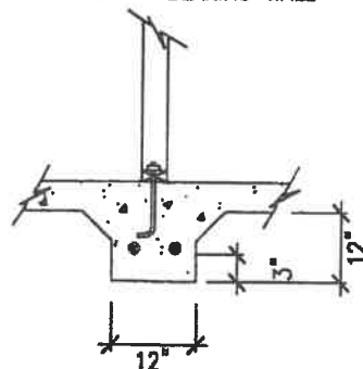
INTERIOR BEARING WALL
