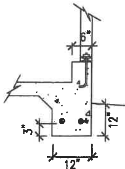
GARAGE RAISED CURB
