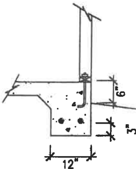
EXTERIOR BEARING WALL
