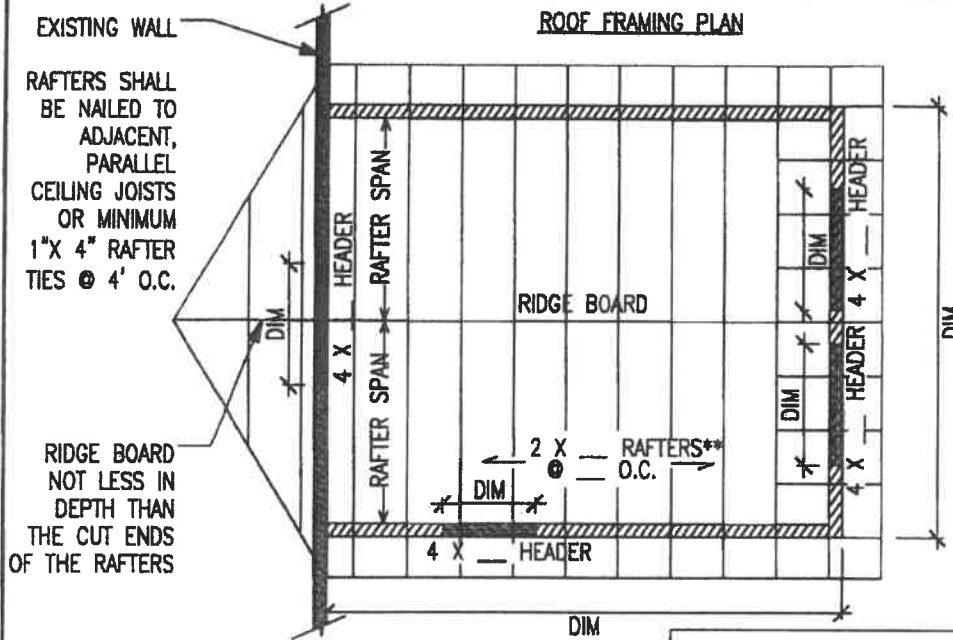
*RAFTERS & JOIST SPAN TABLE BASED ON DOUGLAS FIR/LARCH #2
